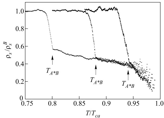
Fig.5. The \rho_s/\rho_s^B ratio for P = 27.97, 22.53 and 16.05 bars (from left to right). Below T_{A^*B} (once the transition is complete) only the B phase is present: thus \rho_s/\rho_s^B = 1 . ( \rho_s^B is a function fitted to the B phase data obtained while warming)
