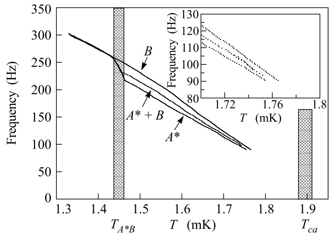
Fig.3. The evolution of the peak frequency of the SM at 27.97 bar. The upper (warming) and lower (cooling) traces depict the B and A^* phase results. The intermediate curve is a history dependent trace obtained by initiating but not carrying to completion the A^* \rightarrow B transition. The inset shows a similar trace obtained by partial penetration into the T_{ca} band. The intermediate frequency SM is evidence for the stable coexistence of the A^* and B phases of ^3\text{He} in 98% aerogel
