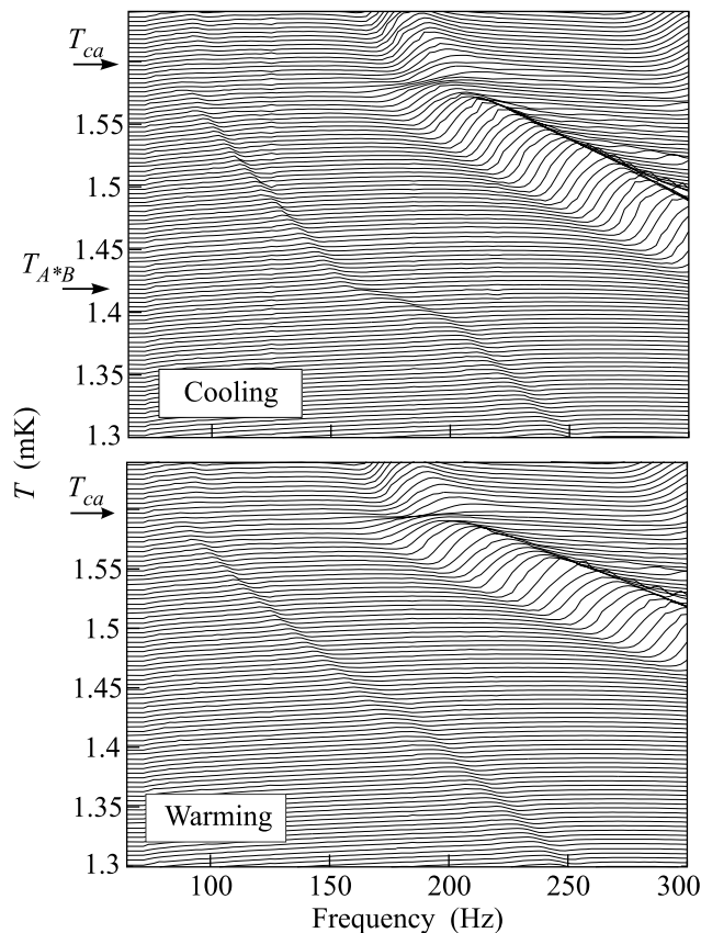
Fig.1. Slow mode (SM) spectra at 21.01 bar offset vertically by temperature (the ordinate displays temperature and the received signal). The positive peak that merges into the weak "edge mode" below 100 Hz at T_{ca} = 1.585\ \text{mK} is the fundamental SM resonance [21]. The broad feature above 170 Hz is a Helmholtz mode combined with SM harmonics that cross close to T_{ca} . The upper panel shows the evolution of the SM on cooling with the A* \rightarrow B transition at T_{A^*B} = 1.415\ \text{mK} . The lower panel depicts the SM behavior on warming
