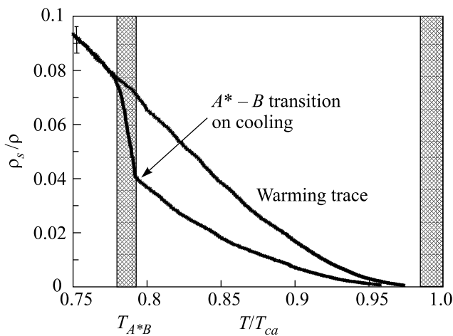
Fig.4. Values of \rho_s/\rho in 98% aerogel at 27.97 bar. The upper curve shows data obtained in the B phase on warming. The lower curve was recorded on cooling, both carried out at \sim 40 \mu\text{K}/\text{hour} . The lower curve shows the signature of the A^* \rightarrow B transition. The cooling and warming traces overlap below the T_{A^*B} “band”
