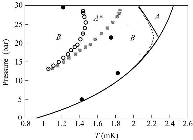
Fig.2. The metastable ^3\text{He} A^* phase in 98% open aerogel in zero magnetic field is bounded by squares that mark the onset of superfluidity ( T_{ca} ), and open circles that mark the A^* \rightarrow B transition observed while cooling. The symbols' width is comparable to the transitions' width. Solid lines show the bulk ^3\text{He} phase diagram in zero field, the dotted line shows the thermodynamically stable bulk B \rightarrow A transition in a 24.9 mT field, and the A \rightarrow B transitions observed in bulk ^3\text{He} in a specially prepared cell (filled circles) [25]. A similar (less pronounced) T_{A^*B} suppression was seen at Northwestern[3]
